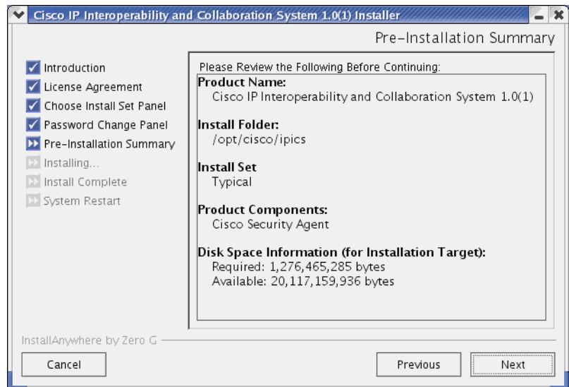
Figure 3-6 Preinstallation Summary
