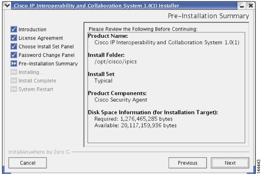
Figure 2-23 Preinstallation Summary
