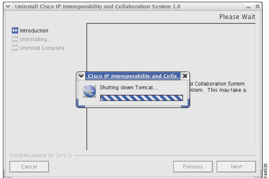
Figure 4-2 Uninstallation Progress
