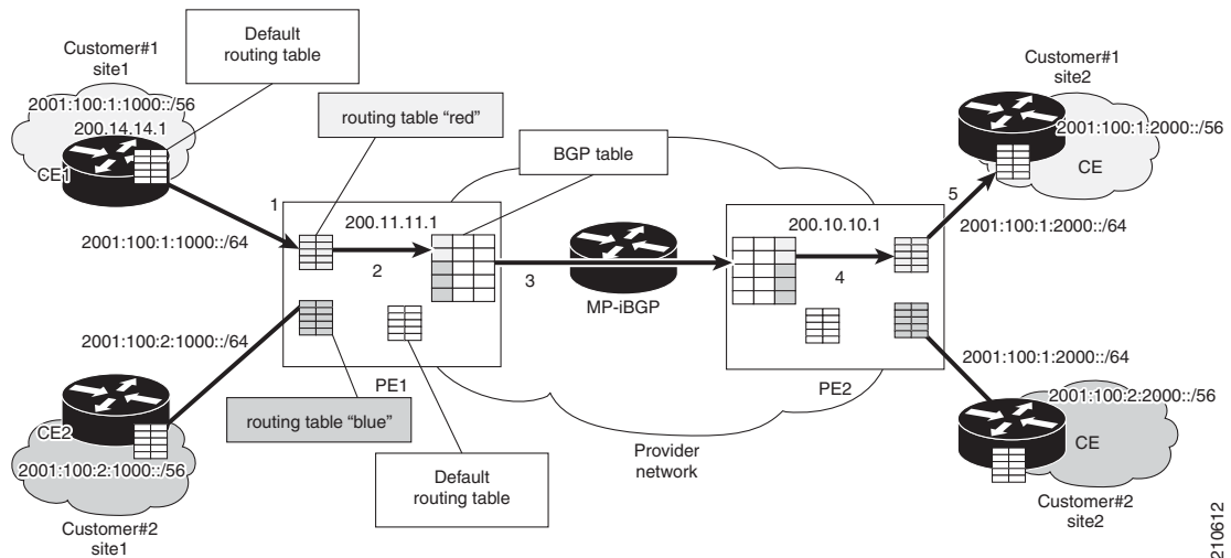
Figure 6-1 6VPE Network Architecture
