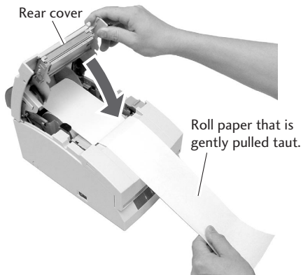
Taking up slack while checking that the copy roll paper winds.
