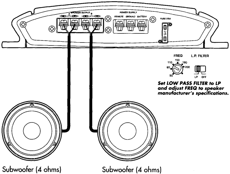
Figure 6. In this application, an APA1100 drives two 4-ohm subwoofers at 150 watts of continuous average power.
