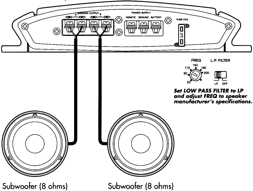
Figure 5. In this application, an APA 1100 drives two 8-ohm subwoofers at 100 watts of continuous average power.
