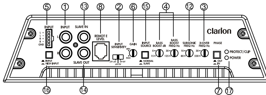
DPX1851 and DPX11551 signal connections and audio adjustments
