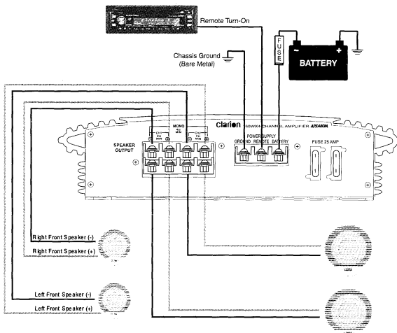
Figure 3 - Electrical connections
