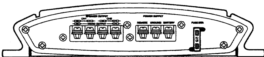
Figure 3. Rear panel layout of the Clarion APA2102.
