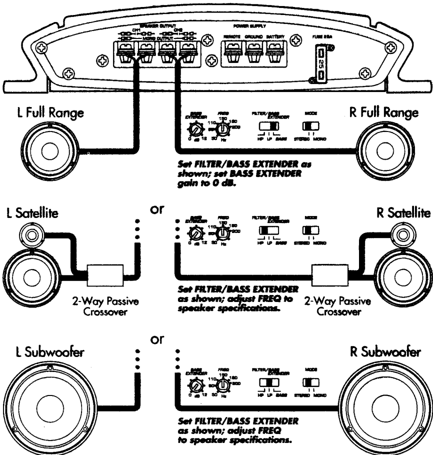
Figure 5. In this application, an APA2102 is used as a 2-channel amplifier that drives two full-range (or satellite or subwoofer) speakers at 50 watts per channel into a 4-ohm load. NOTE: A passive crossover must be used with satellite speakers.
