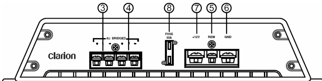
APX2121E power and speaker connections
