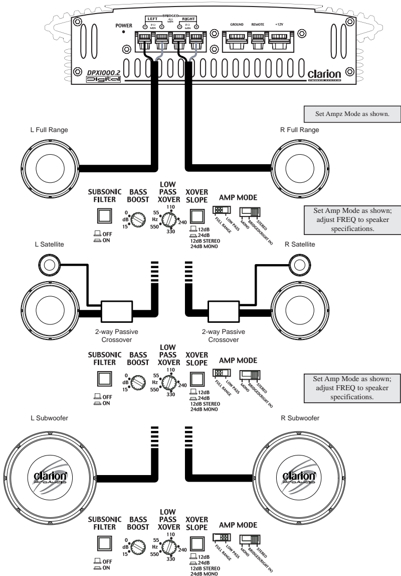
Figure 4 - In this application, the amplifier is used in stereo and drives two full-range (or satellite or subwoofer) speakers. NOTE: A passive crossover must be used with satellite speakers. Minimum load in the stereo mode is 1 ohms.
