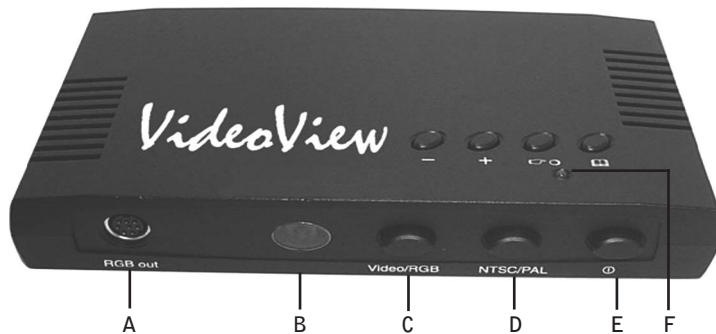
Figure 1. Front panel
