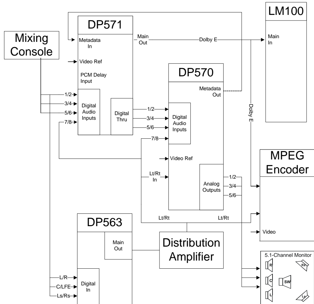
Figure 6-1 Typical Live Remote Transmission Setup
