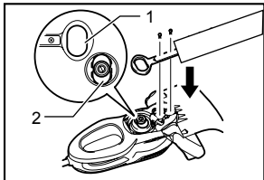
1. Ellipse of shear blade 2. Crank
