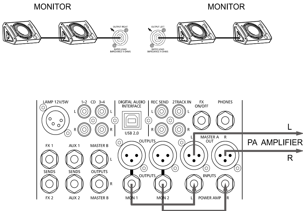
Illustration 6-3: Using internal power amplifier for monitoring purposes
