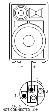
Illustration 2-20: Connection of a passive speaker
