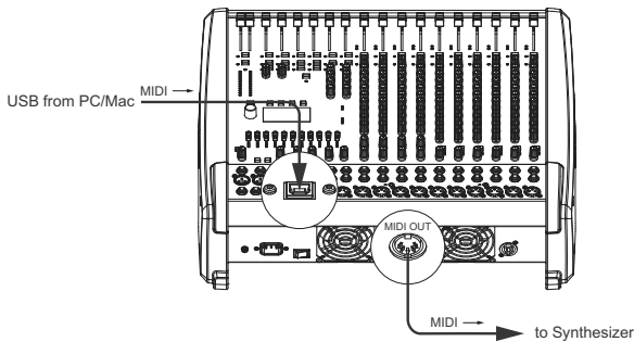
Illustration 4-4: Sending MIDI data from a PC/Mac to a Synthesizer
