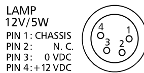
Illustration 2-18: Pin assignment of LAMP 12V/5W output
