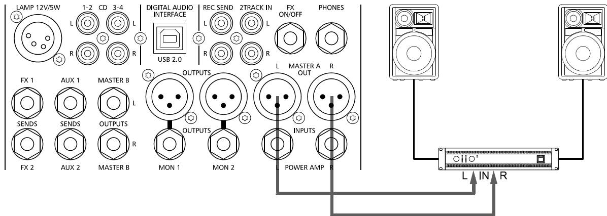
Illustration 6-2: Connection of an external power amplifier at MASTER A OUT L/R
