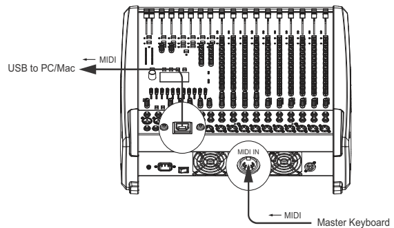
Illustration 4-5: Sending MIDI data from a Master Keyboard to a PC/Mac
