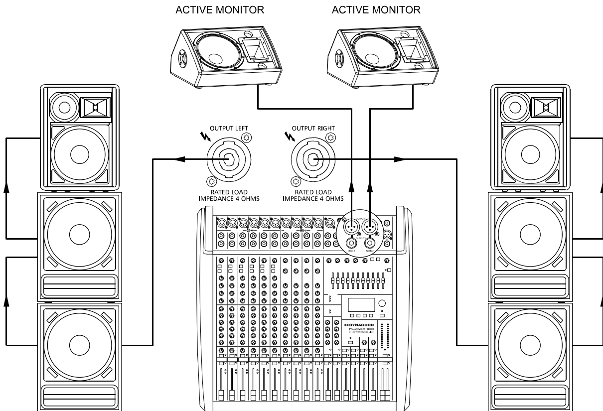
Illustration 6-1: Maximum amount of speakers in passive configuration
