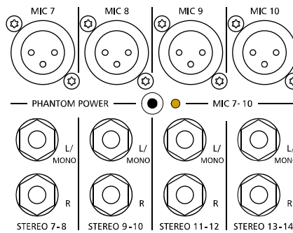
Illustration 2-9: Microphone input (Stereo) of PowerMate 1000
