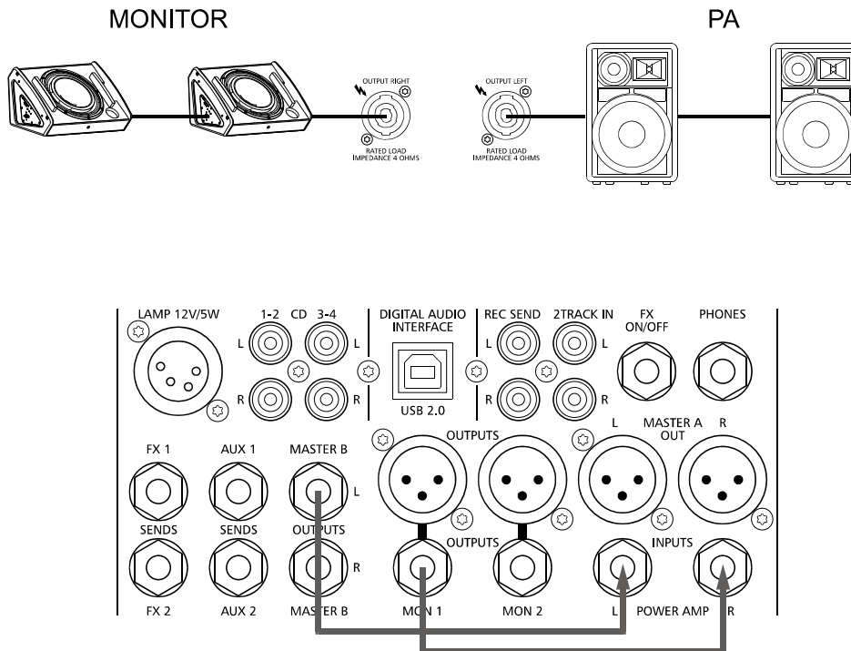
Illustration 6-4: Mono PA + Monitor
