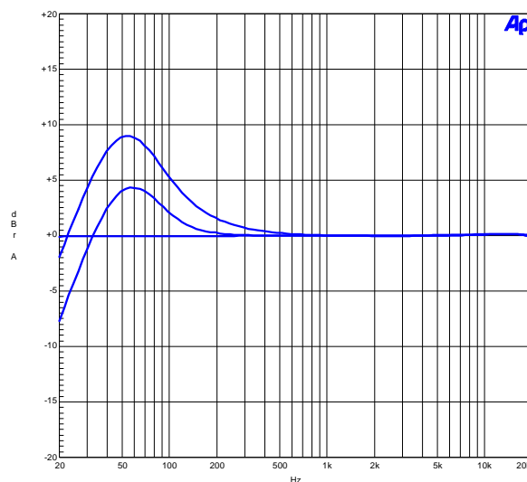
Illustration 2-19: Frequency plot of LPN filters for settings High, Medium or Flat
