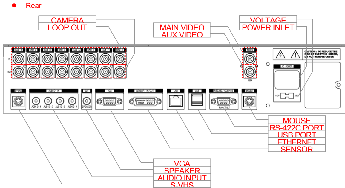
[Fig 5-2. Rear View]
