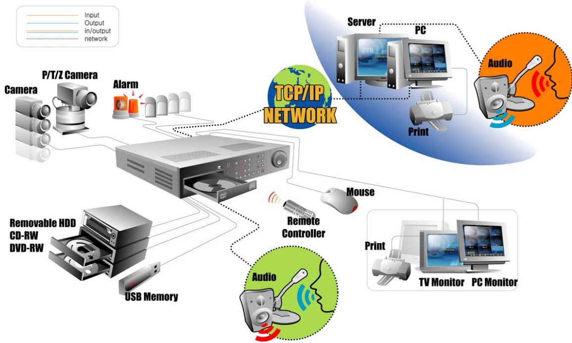
[Fig 5-3. System Connection]
