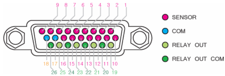
[Fig 5-6. SENSOR IN/OUT PIN]
