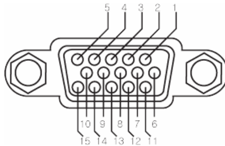
[Fig 5-5. VGA Connector PIN]
