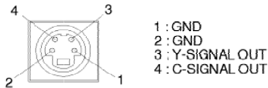
[Fig 5-4. S-VHS Connector PIN]
