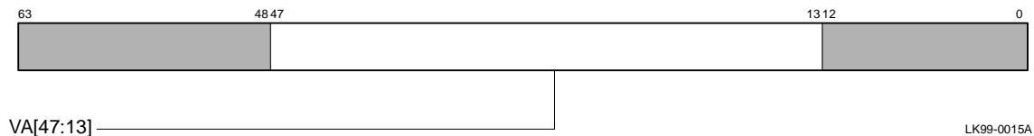
Figure 5–8 ITB Tag Array Write Register
