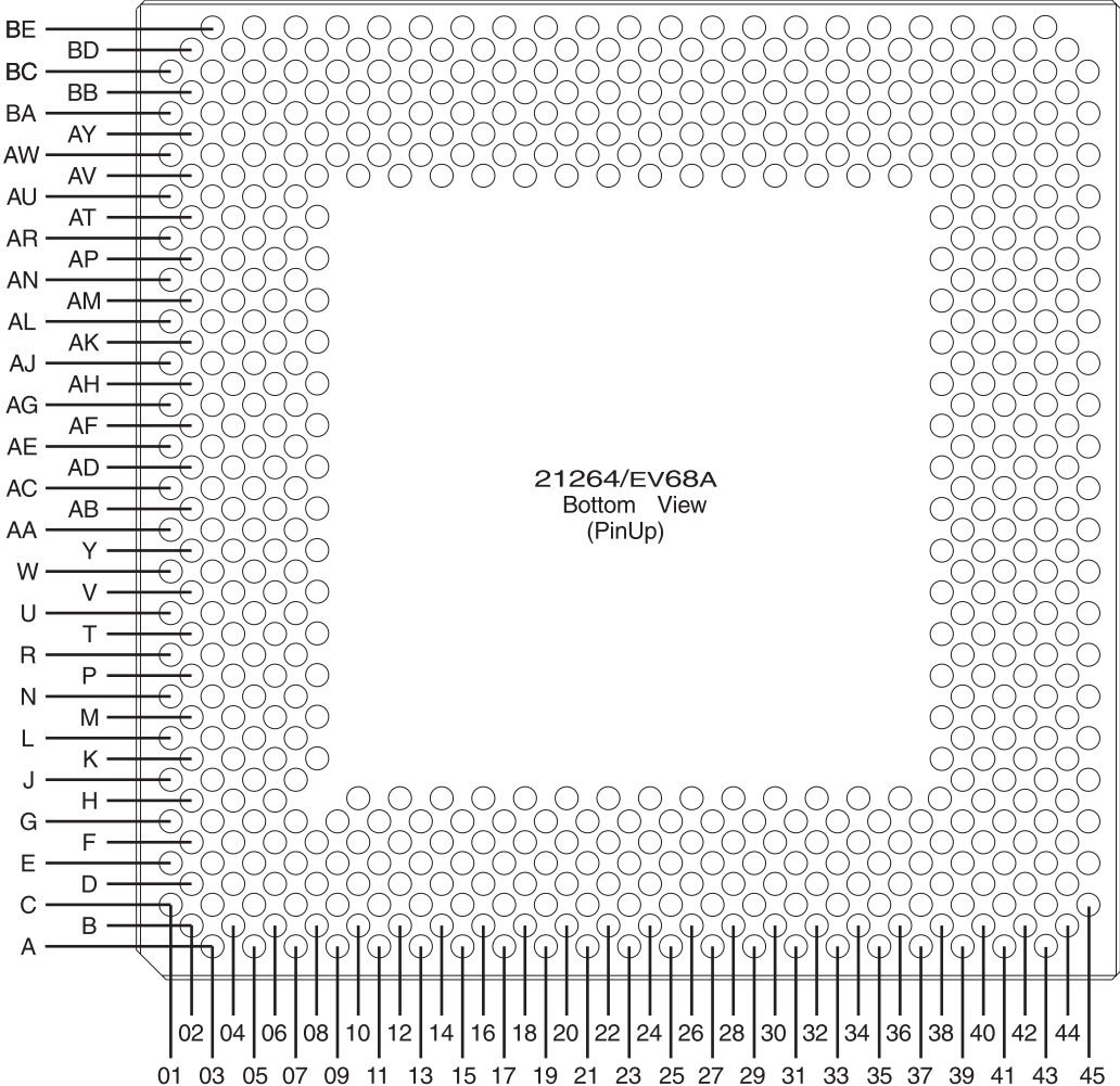
Figure 3-4 21264/EV68A Bottom View (Pin Up)
