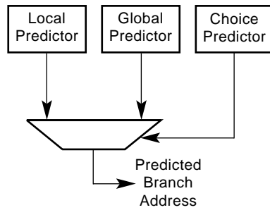
Figure 2–2 Branch Predictor
