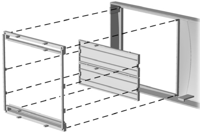
Removing the Subpanel and Bezel Blanks
