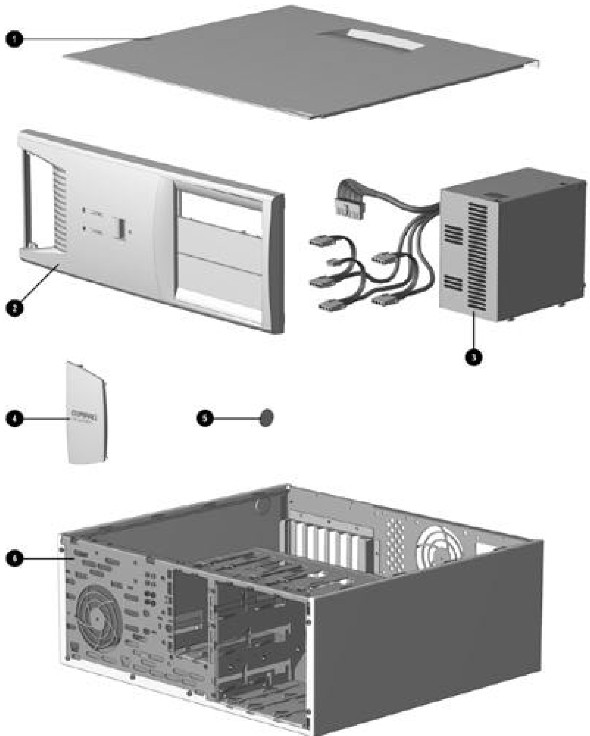
System Unit Spare Parts - Intel 810/810e Model
