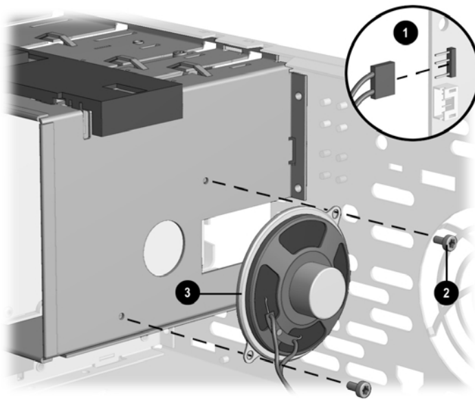
Removing the Speaker From the Side of the Drive Cage
