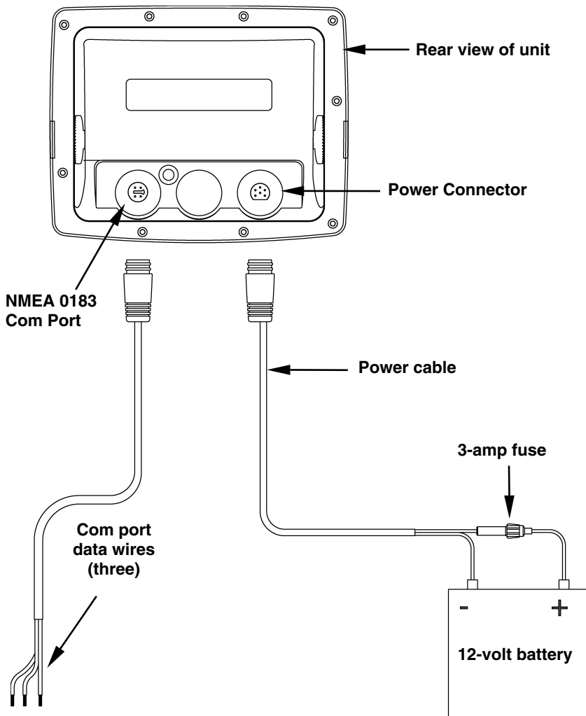
Cable connections.
