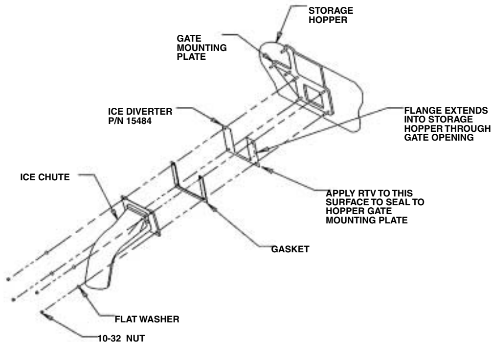
FIGURE 1. Exploded View of Ice Diverter Installation
