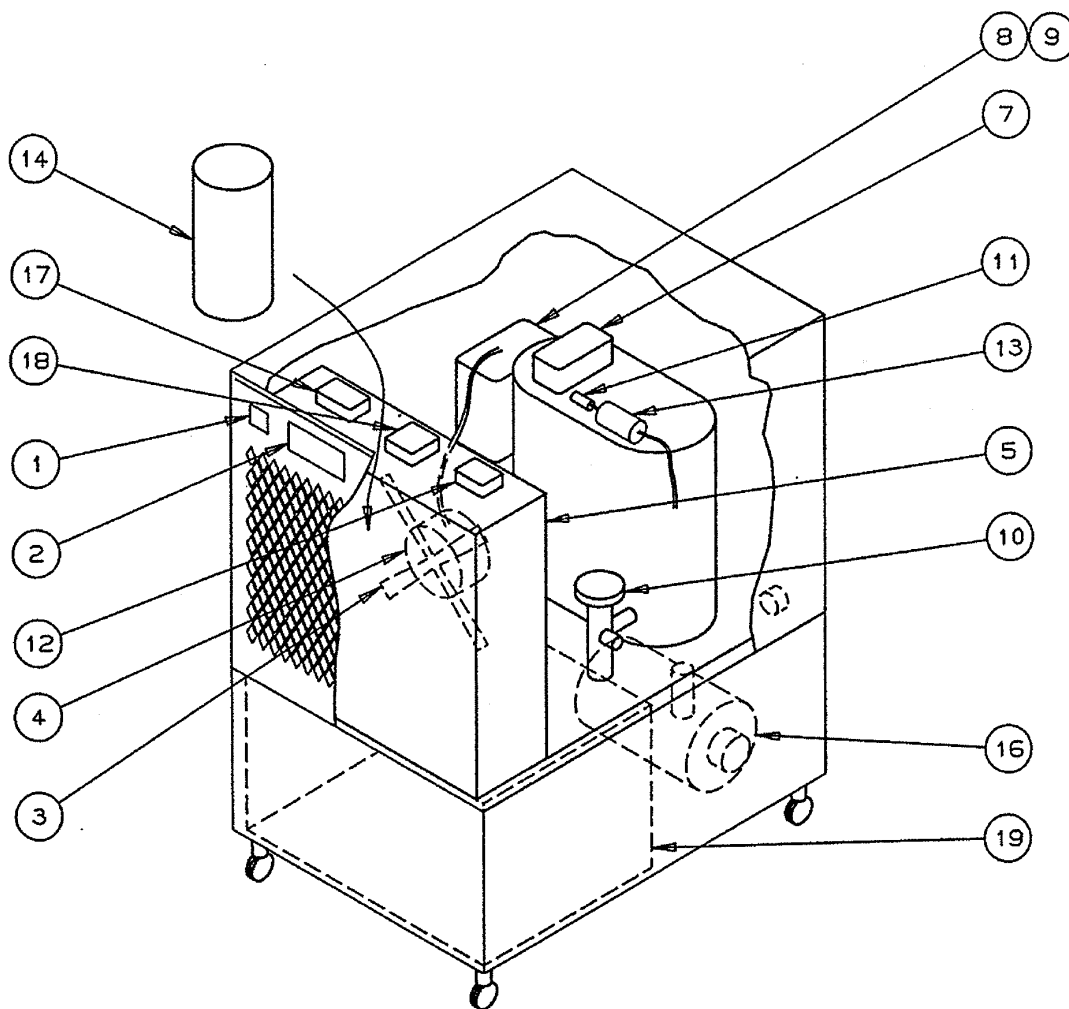
FIGURE 1. CH750, CH751 AND CH951 EXPLODED VIEW
