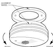
D: Installation / Removal
