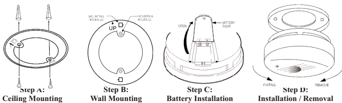
Figure 2: Installation Instructions
