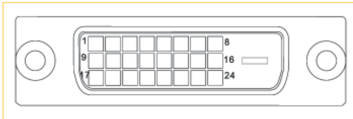
DVI Connector
