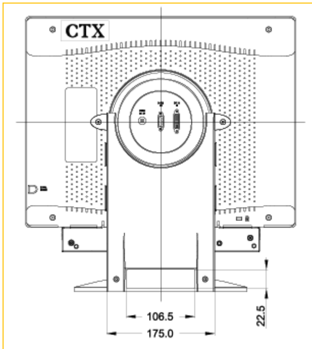
Rear View (unit: mm)
