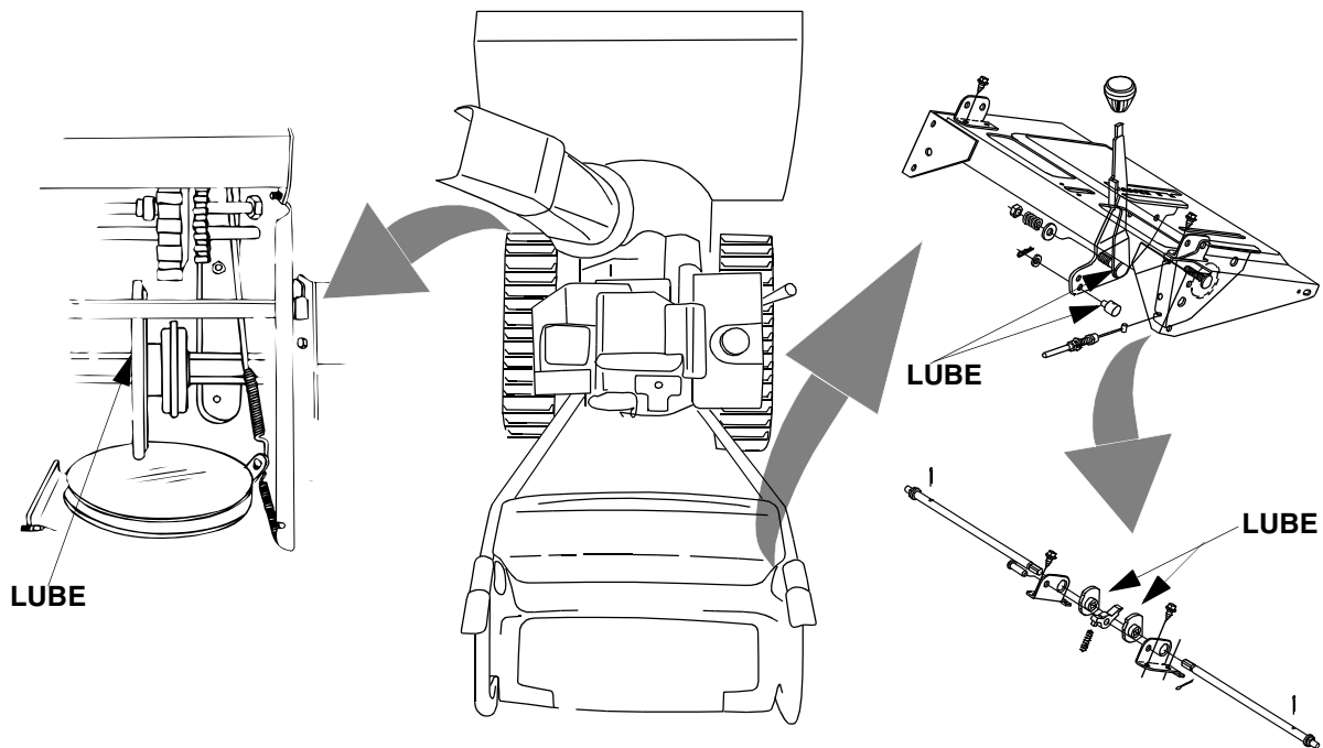
Figure 20: Lubrication Chart
