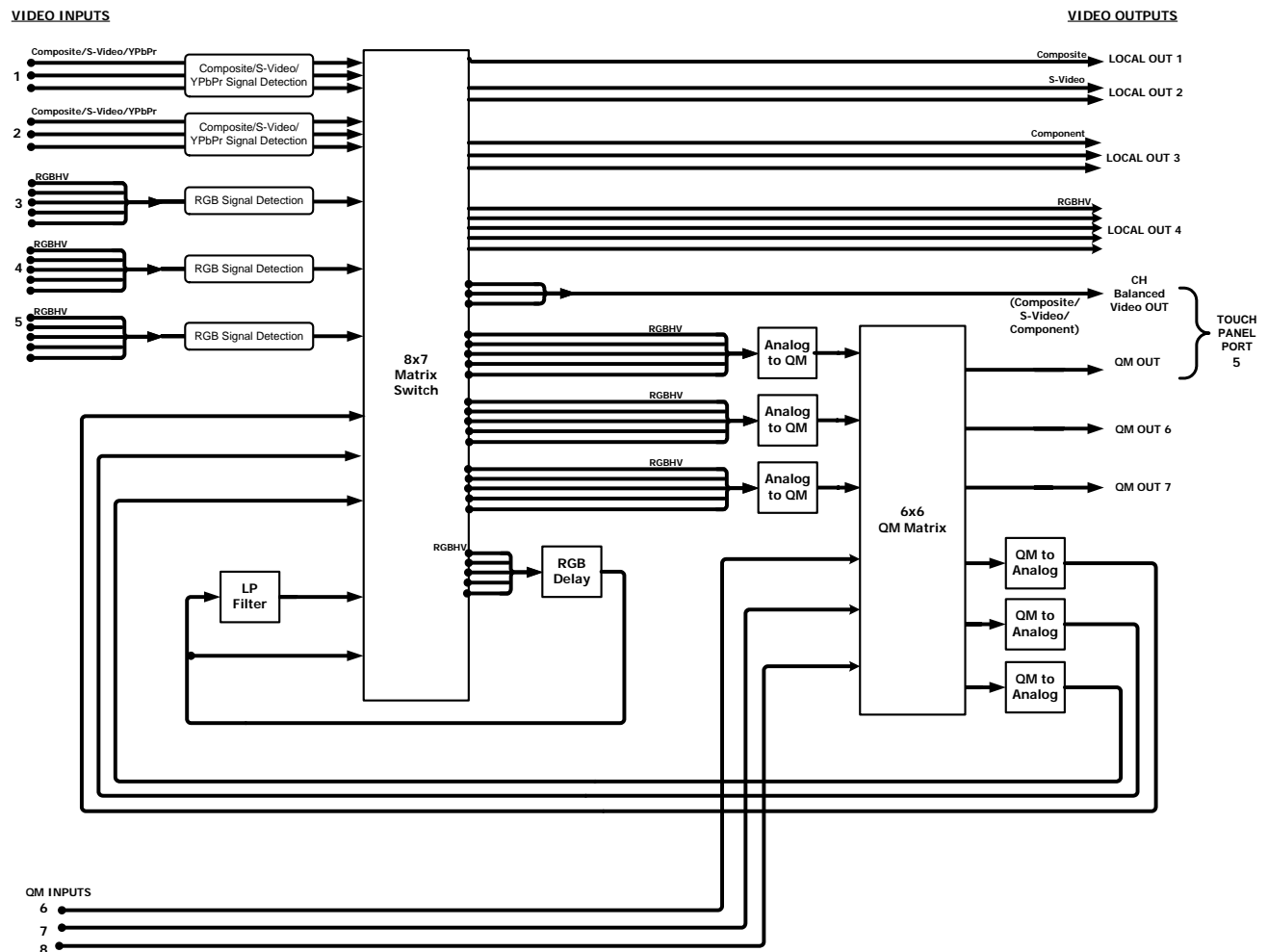
Video Block Diagram of the MPS-300
