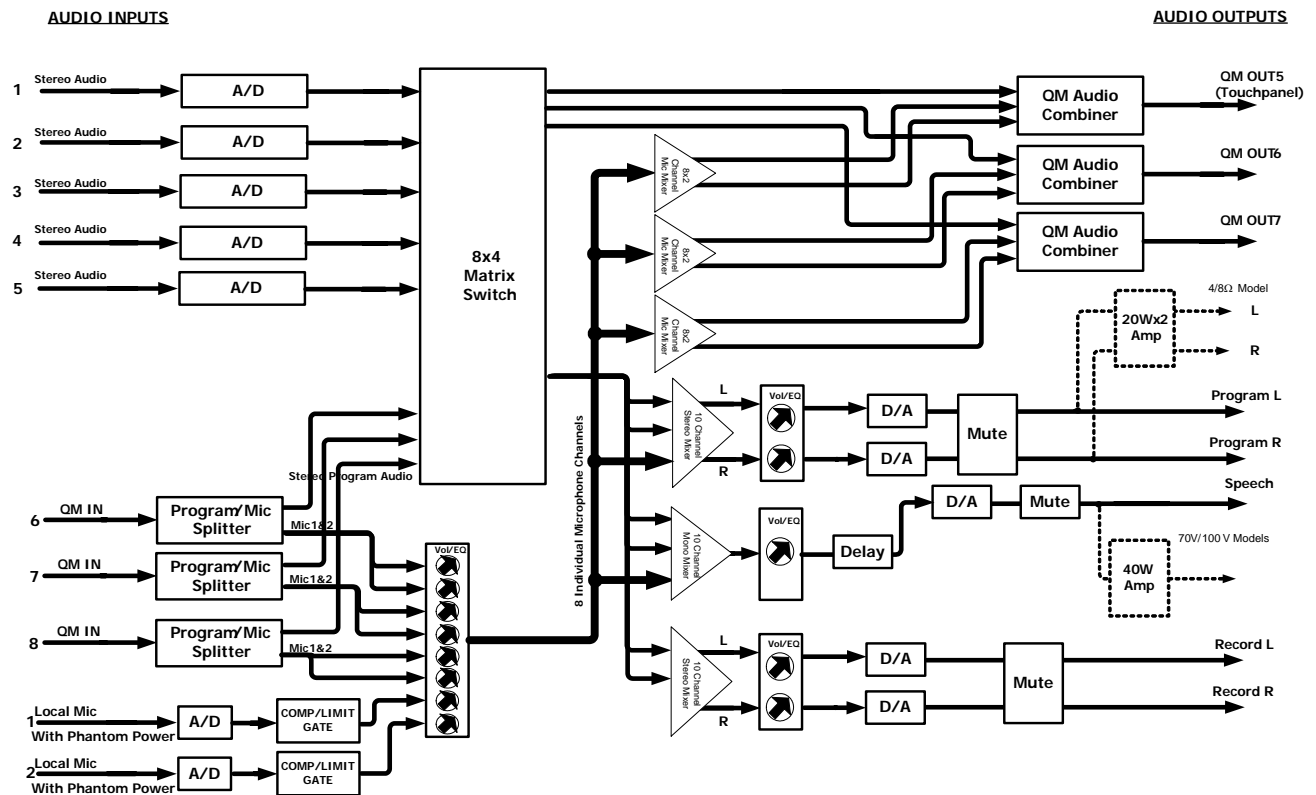
Audio Block Diagram of the MPS-300
