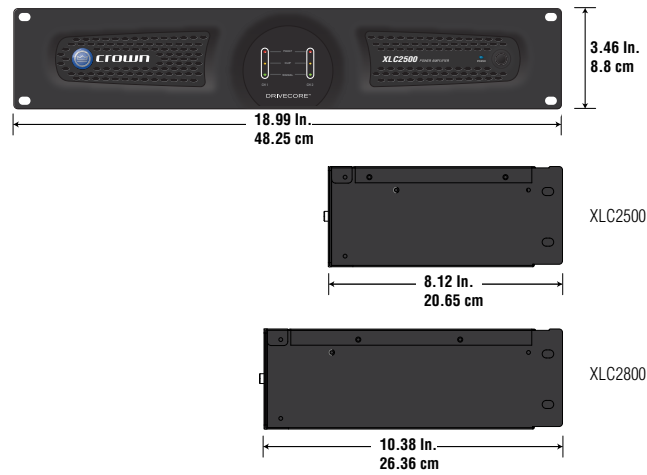
Figure 2.2 Dimensions
