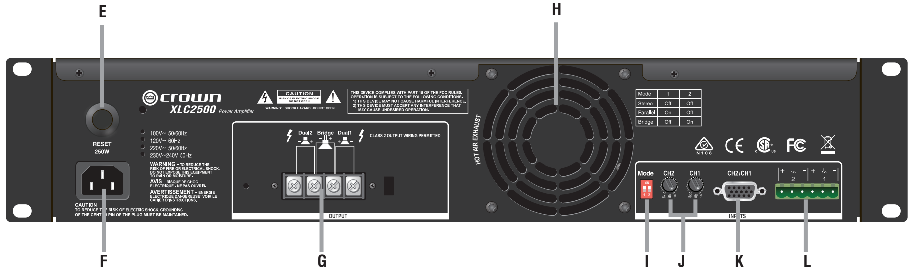
Figure 3.2 Rear Panel 图3.2 后面板
