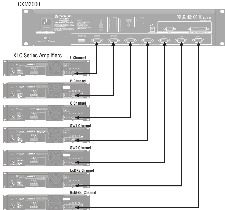
Figure 2.4 Wiring XLC Amplifiers to the CXM2000 in Bi-amplified Cinema Speakers System 图 2.4 双功放通道驱动式扬声器系统中XLC功放与CXM2000的连接
