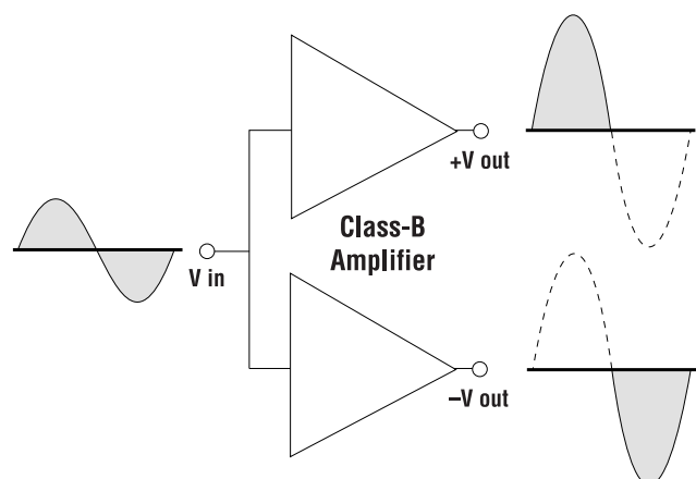
Class-B Operation
