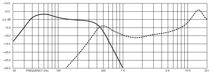
Frequency Response
