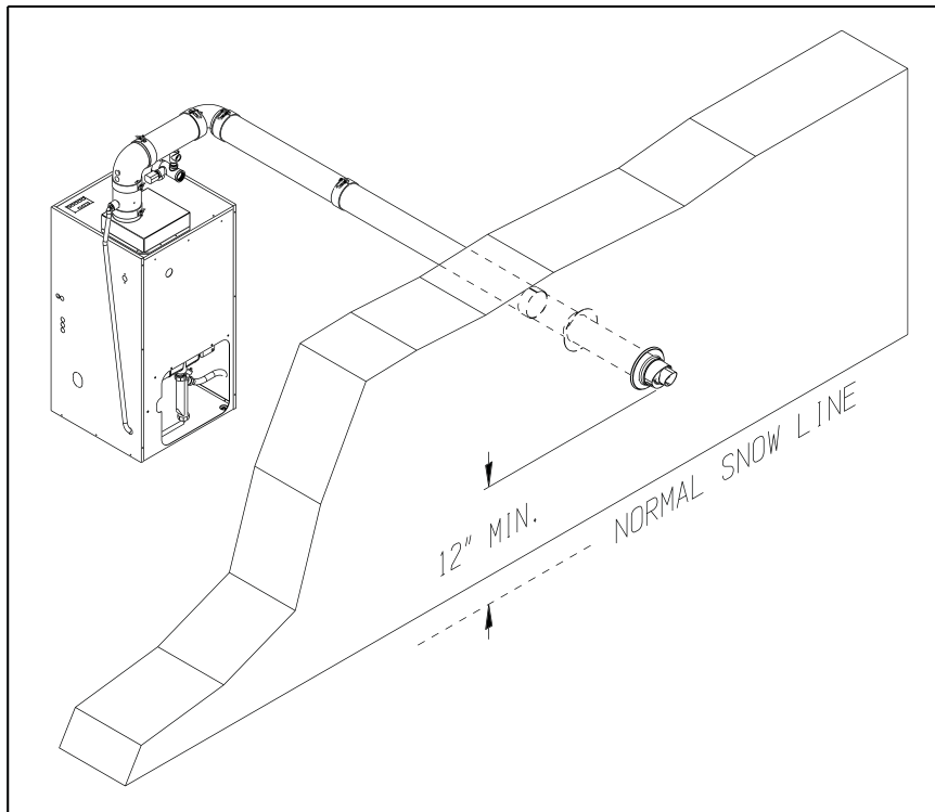
FIGURE 1.2: HORIZONTAL CONCENTRIC VENTING (VENT OPTION 3,4)
