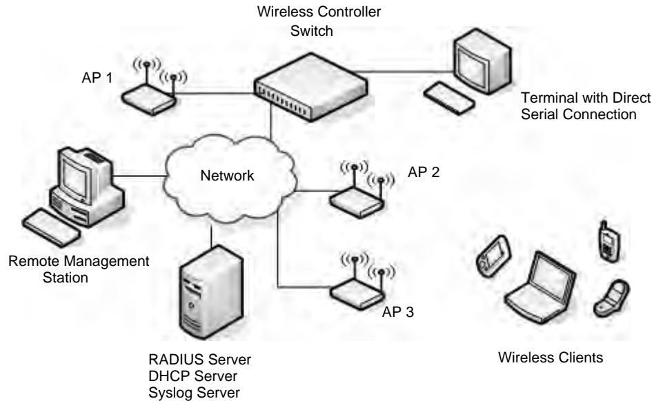
Figure 7. D-Link Unified Access System Components
