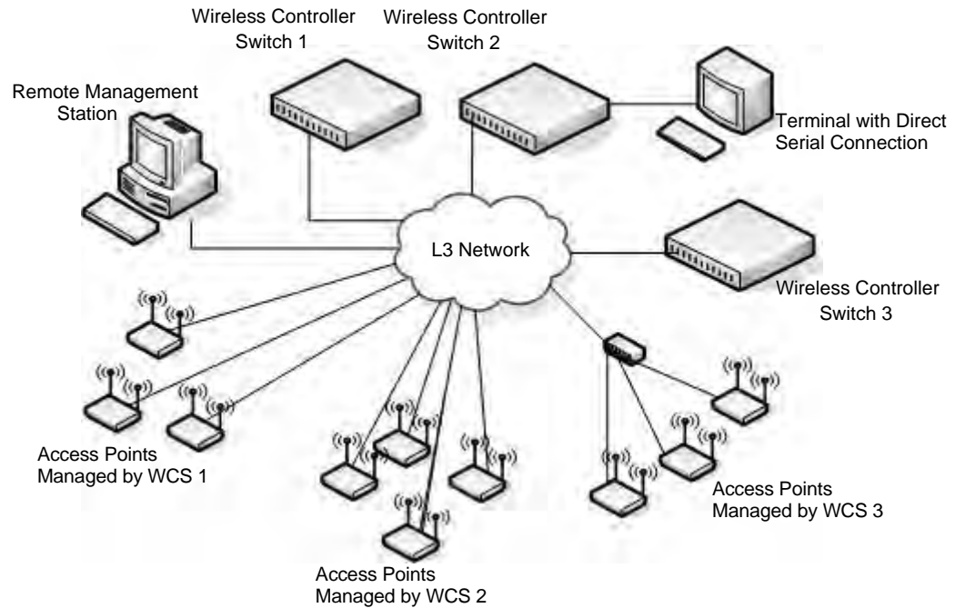
Figure 3. Peer WCS with Layer 3 Roaming Support
