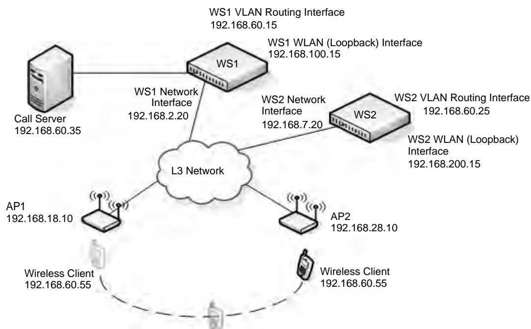
Figure 83. Example of a Network with L3 Tunnel Subnet
