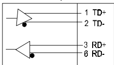
PC Board
