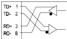
RJ-45 Connector/ Receptacle
