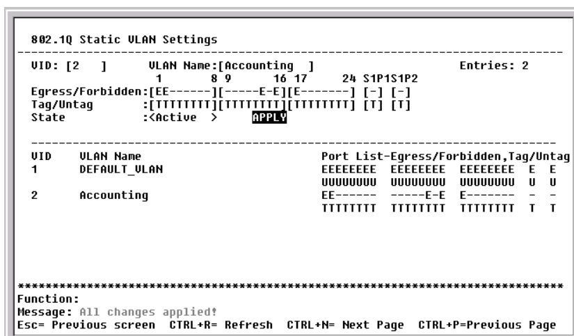
Figure 6-25. 802.1Q Static VLAN Settings screen
