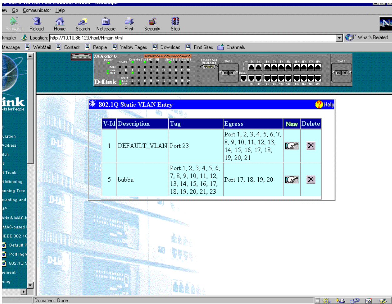
Figure 7-27. 802.1Q Static VLAN Entry window (number one)
