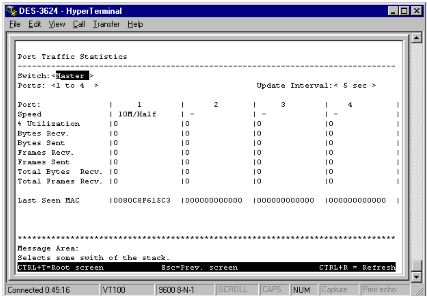
Figure 6-47. Port Traffic Statistics screen
