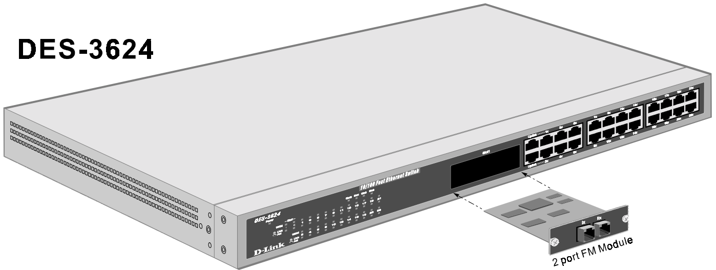
Figure 3-6. Two-port, 100BASE-FX (MT-RJ) module
