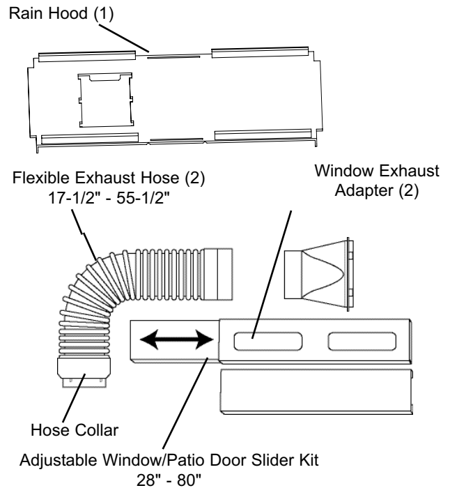
Fig. 1 Installation Accessories Rain Hood Inserts (2)
