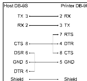
Part # 32-2300-01
