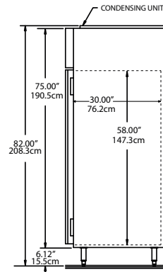
END VIEW 2 & 3 SECTION UNITS
