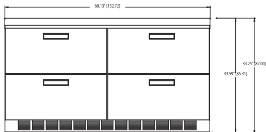
UCD4460N ELEVATION VIEW
