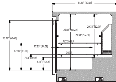
UC4460N RIGHT SIDE VIEW
