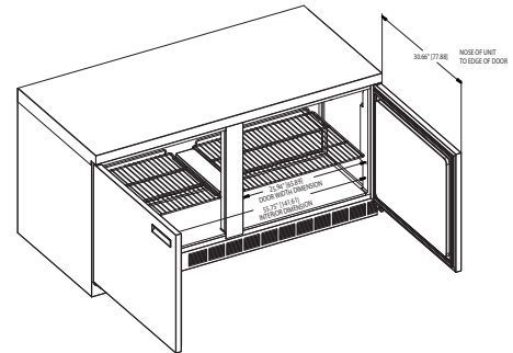
UC4460N ISO VIEW
