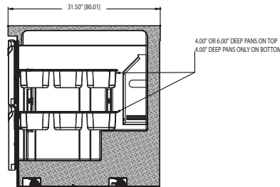
UCD4460N RIGHT SIDE VIEW
