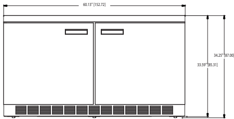
UC4460N ELEVATION VIEW
