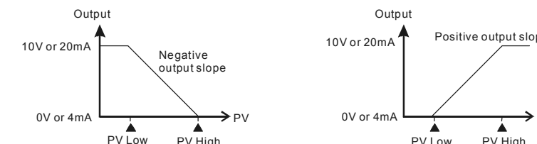
Figure 7: Proportional Output
