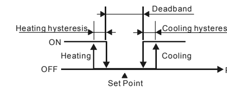
Figure 4: ON/OFF Control
