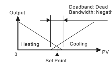
Figure 6: PID Control
