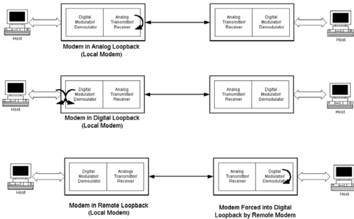
Figure 2-4. Loopback Diagnostics
