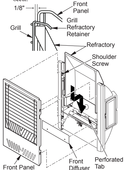
Figure 15 - Installing Front Panel and Refractory
