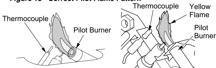
Figure 19 - Incorrect Pilot Flame Pattern
