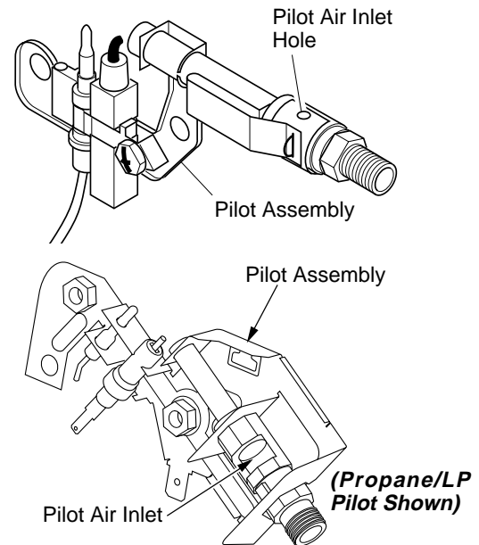
Figure 22 - Pilot Inlet Air Hole
