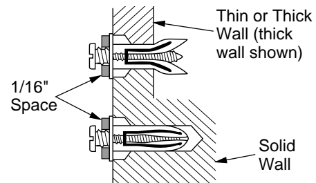
Figure 6 - Tightening Anchors
