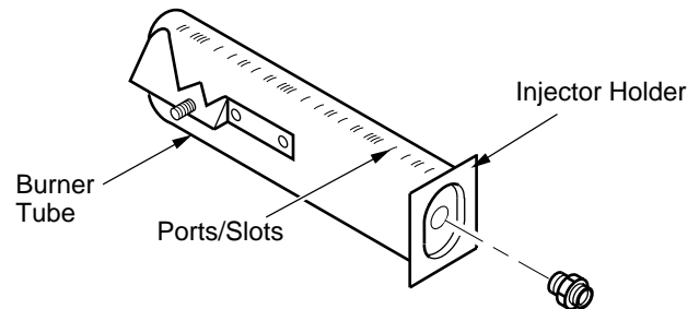
Figure 23 - Injector Holder On Burner Tube
