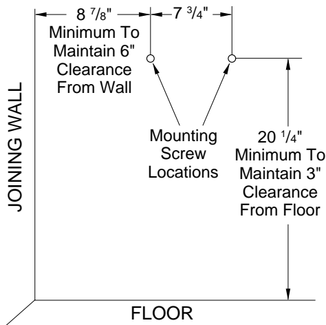
Figure 3 - Mounting Screw Locations
