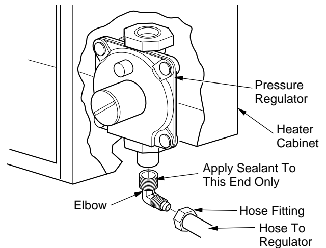
Figure 10 - Gas Connection
