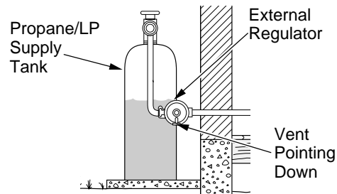
Figure 12 - External Regulator With Vent Pointing Down
