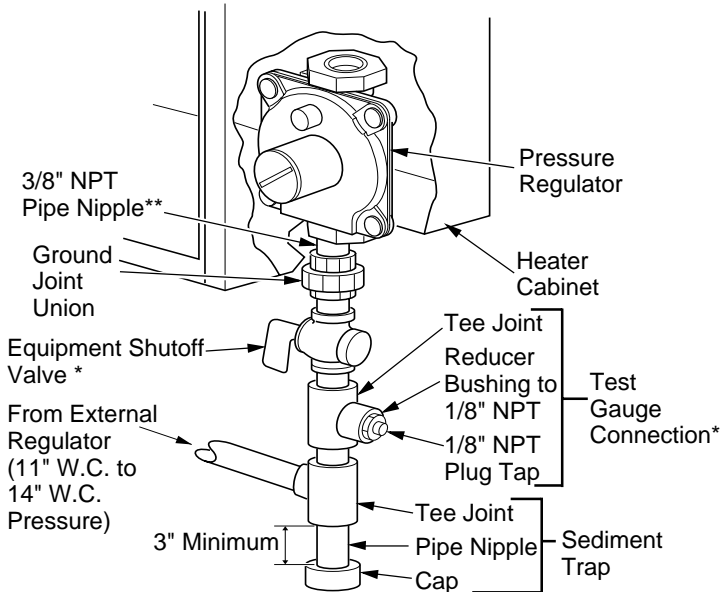
Figure 13 - Gas Connection
