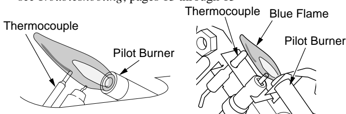
Figure 18 - Correct Pilot Flame Pattern
