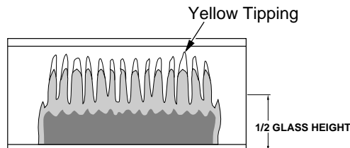
Figure 21 - Incorrect Burner Flame Pattern
