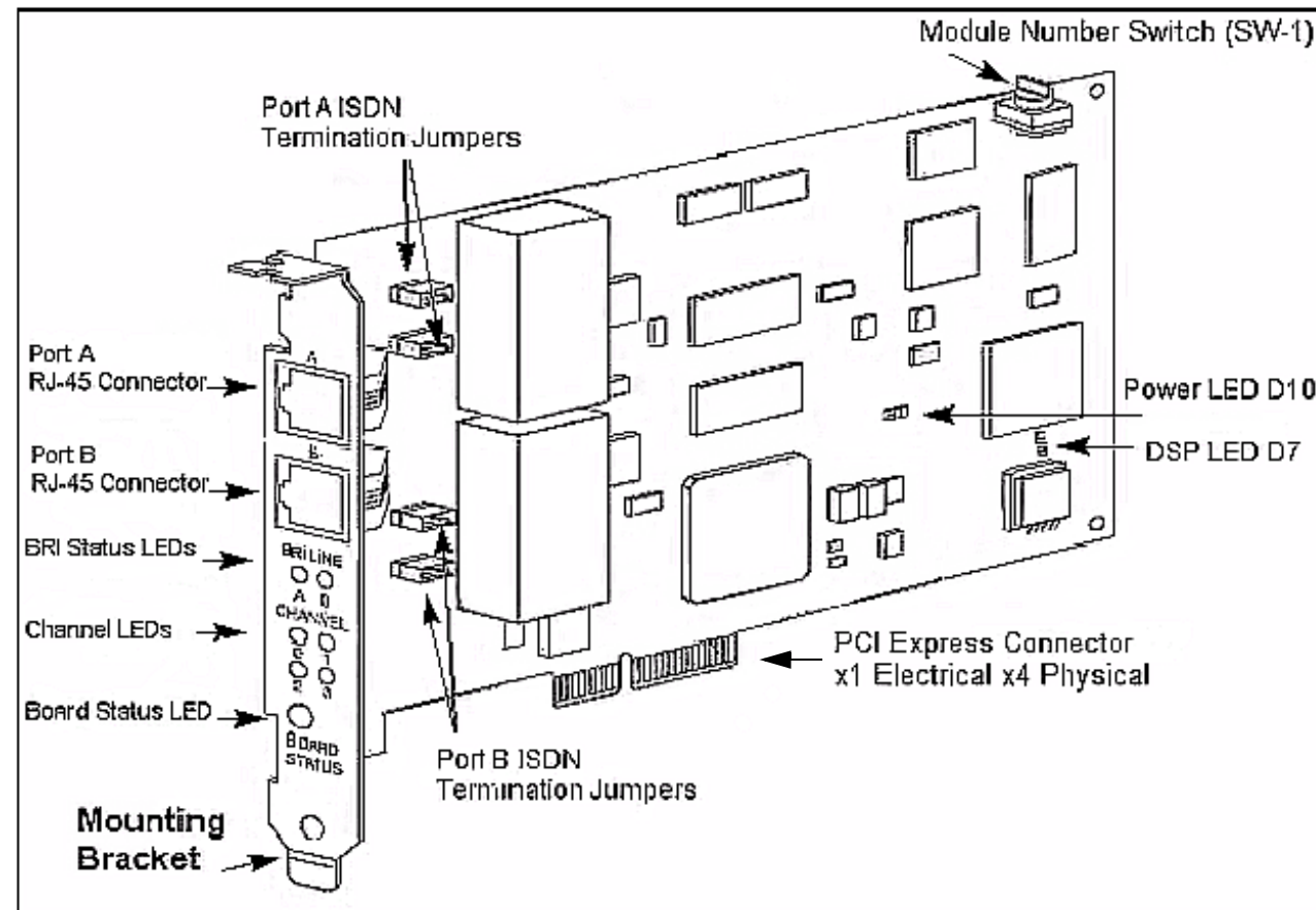
Figure 5. TR1034 BRI PCI Express Series Board
