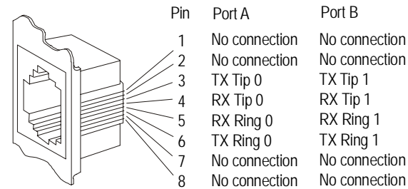
Figure 4. Connector Pinouts
