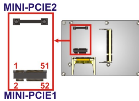
Figure 3-15: PCIe Mini Card Slot Location
