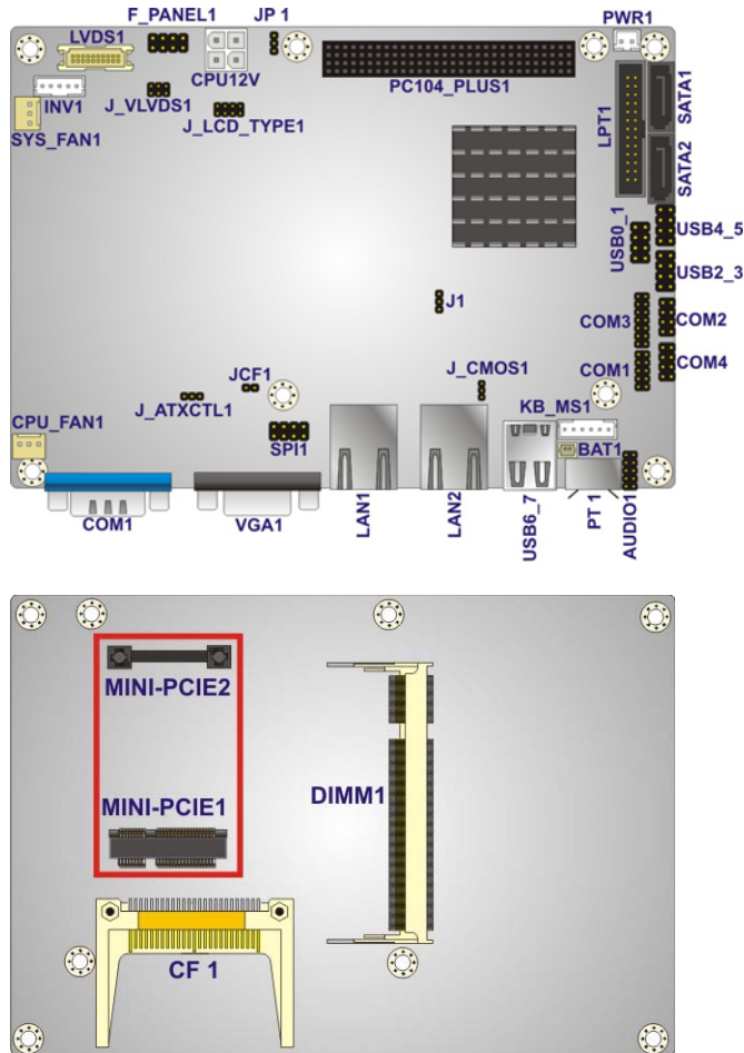
Figure 1-2: Connectors
