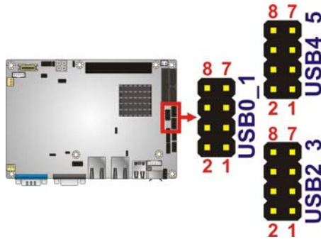
Figure 3-21: USB Connector Pinout Locations
