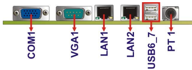
Figure 3-22: External Peripheral Interface Connector
