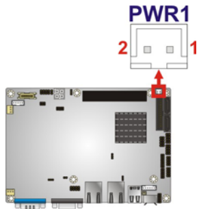
Figure 3-17: SATA Power Connector Locations
