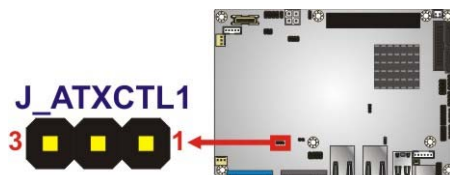
Figure 4-4: AT/ATX Power Select Jumper Settings
