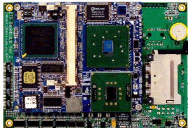
Underside of Neptune showing ETX CPU module
