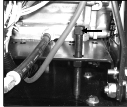
Figure 36: Tension Bolt
