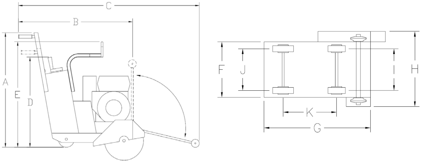
Figure 3: CC1800XL Dimensions
