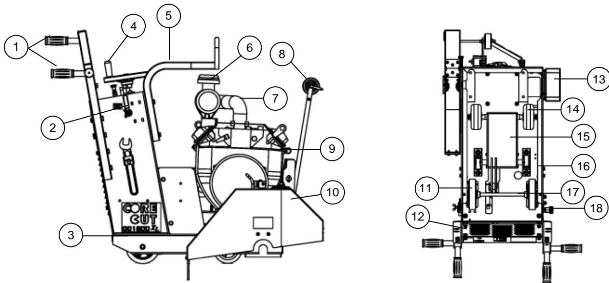
Figure 1: CC1800XL Components
