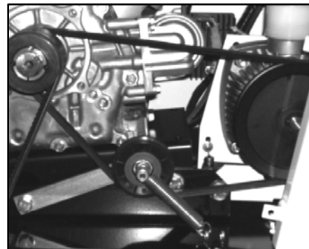
Figure 37: Transmission V-Belt
