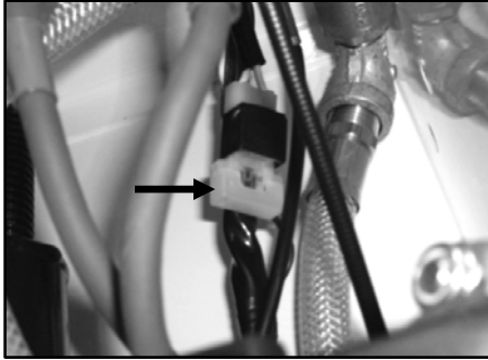
Figure 29: In-Line Fuse
