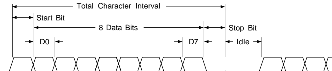
Figure 3. Bit Timing Diagram
