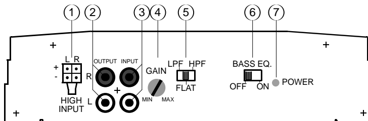
FIGURE 1—AMPLIFIER CONNECTIONS 200/2 - 300/2 FRONT
