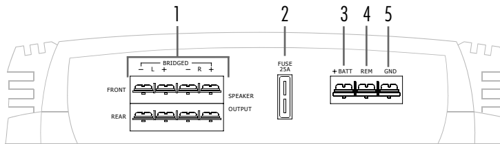
FIGURE 2—AMPLIFIER CONNECTIONS 250/4 REAR
