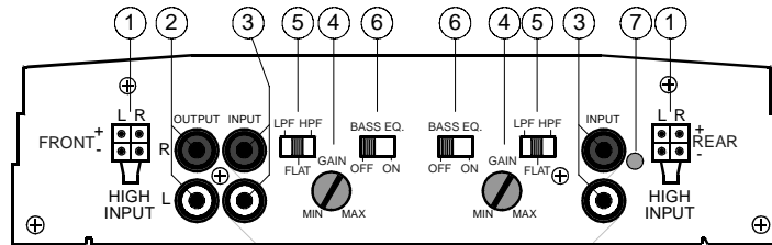
FIGURE 2—AMPLIFIER CONNECTIONS 250/4 FRONT
