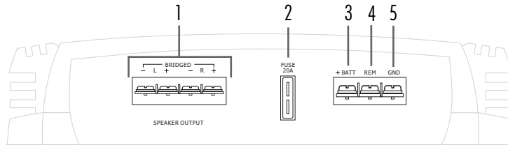
FIGURE 2—AMPLIFIER CONNECTIONS 200/2 300/2 REAR
