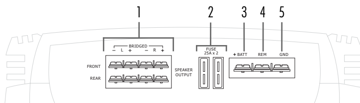
FIGURE 2—AMPLIFIER CONNECTIONS 600/4 REAR
