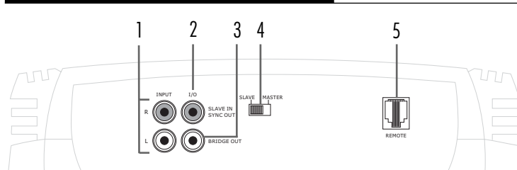
FIGURE 1—AMPLIFIER CONNECTIONS 750d/1500d FRONT
