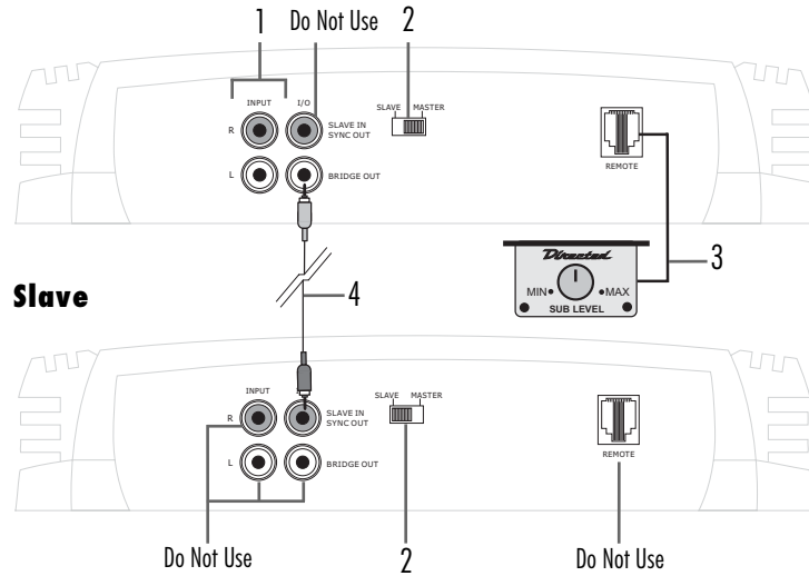
FIGURE 6—EXTERNAL SYNC BRIDGED 750d/1500d
