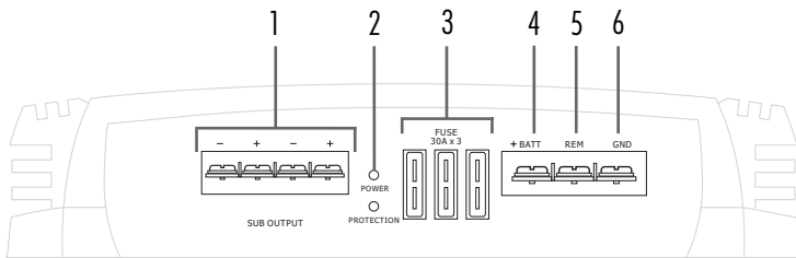
FIGURE 3—AMPLIFIER CONNECTIONS 1500d REAR
