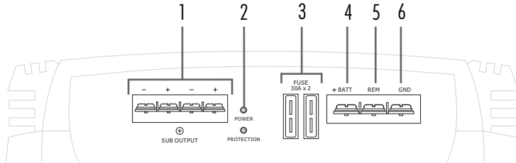
FIGURE 2—AMPLIFIER CONNECTIONS 750d REAR
