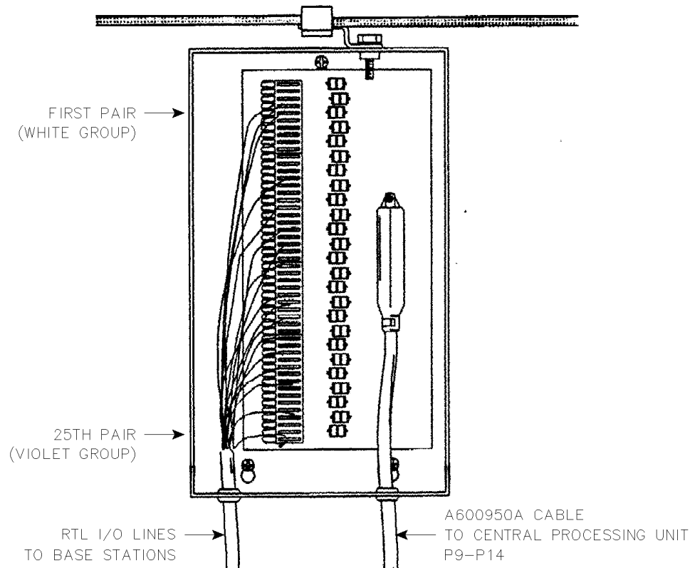
Figure 2-12 SURGE ARRESTOR BOX WIRING
