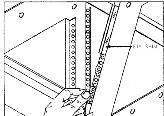
Figure 3-17 INSTALLING TINNERMAN CLIPS
