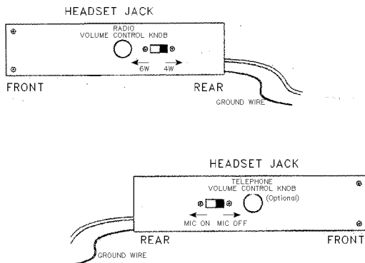
Figure 5-7 CONNECTOR HEADSET
