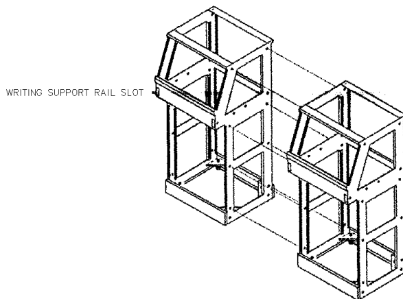
Figure 3-3 ASSEMBLY OF CONSOLE SECTIONS
