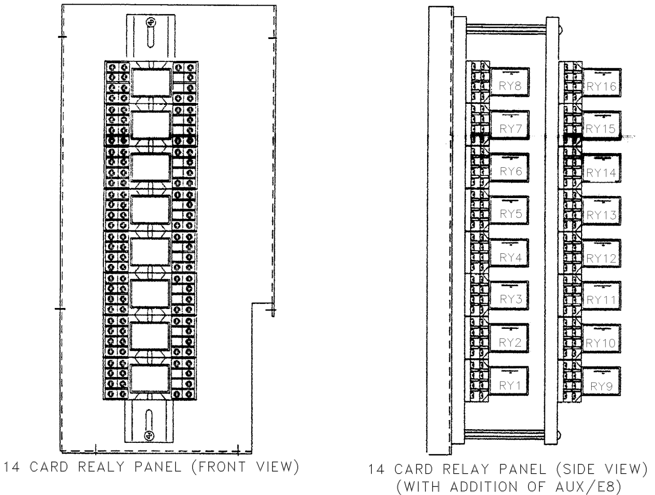
Figure 2-14 14 CARD RELAY PANEL
