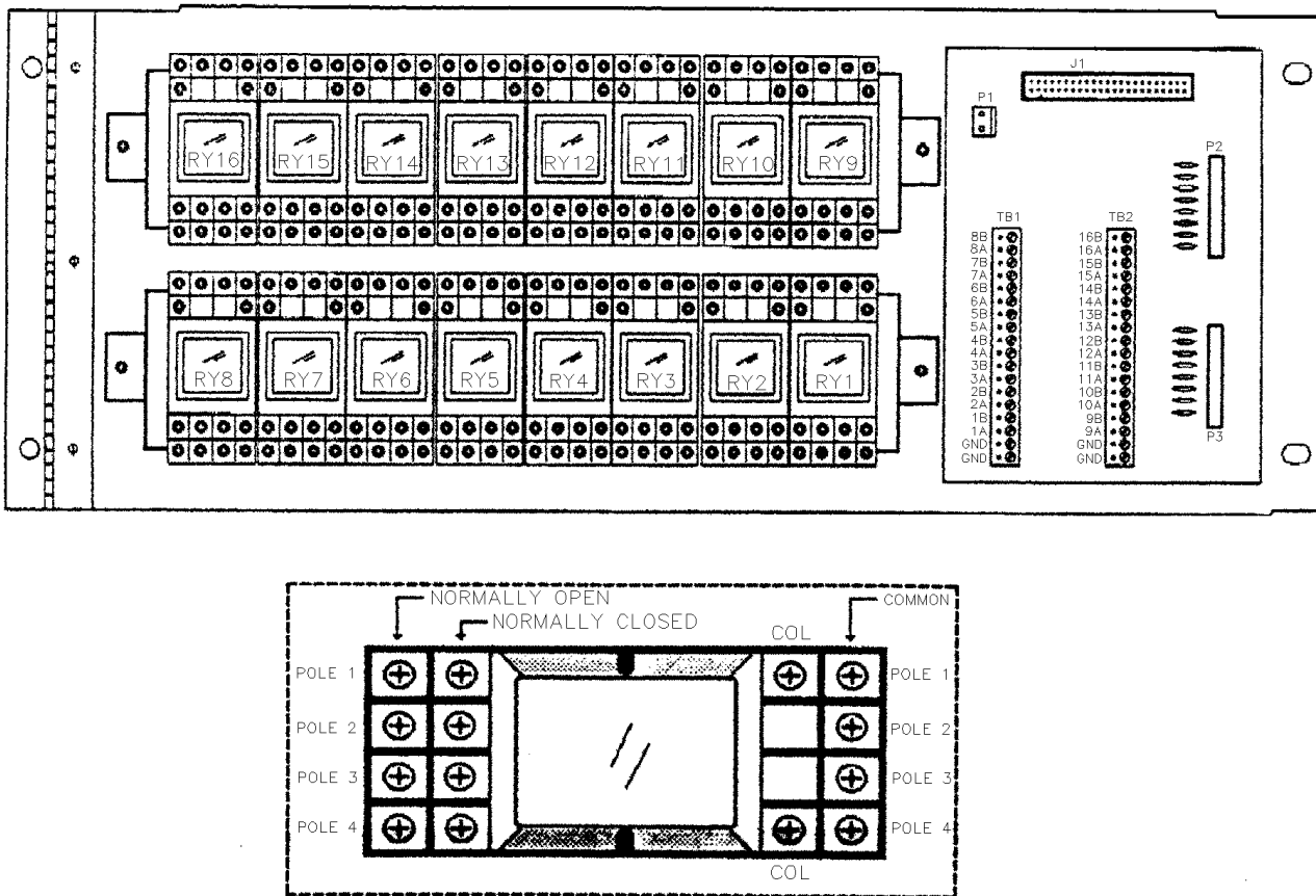
Figure 2-13 CPU RELAY PANEL
