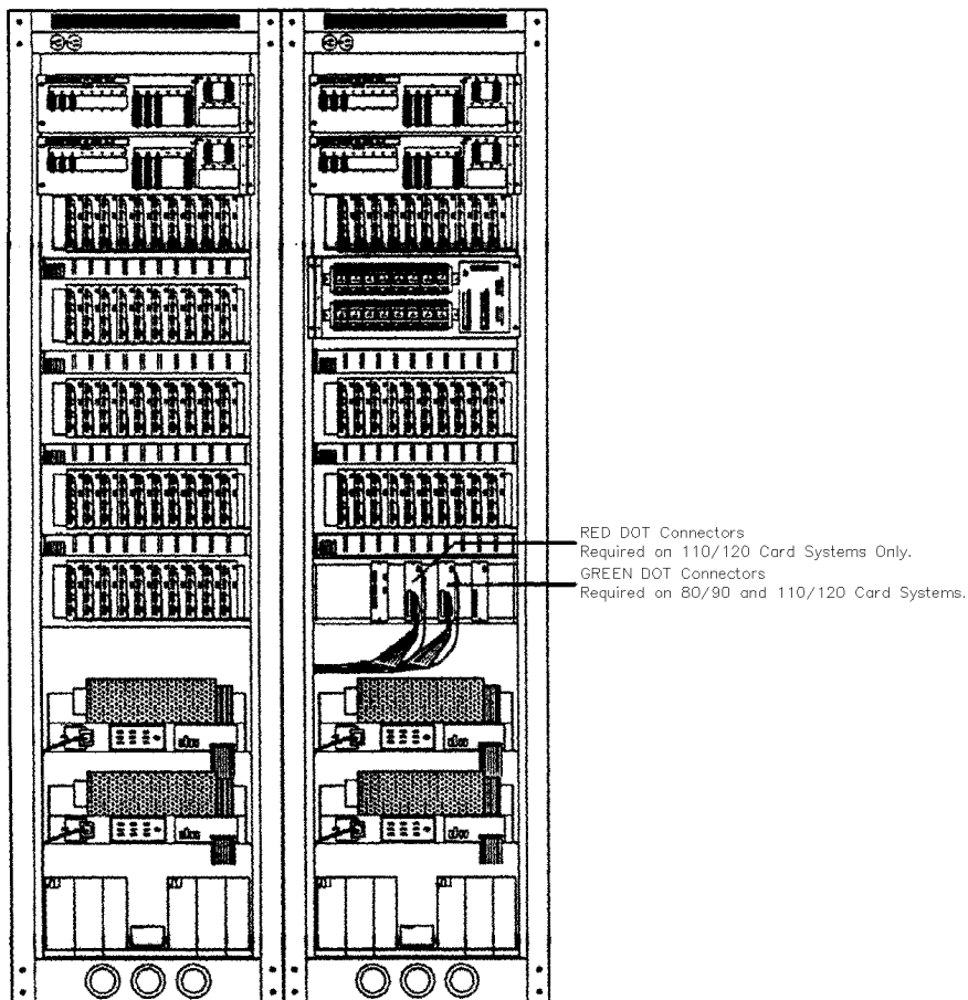
Figure 2-2 CPU CABINET CABLE CONNECTIONS
