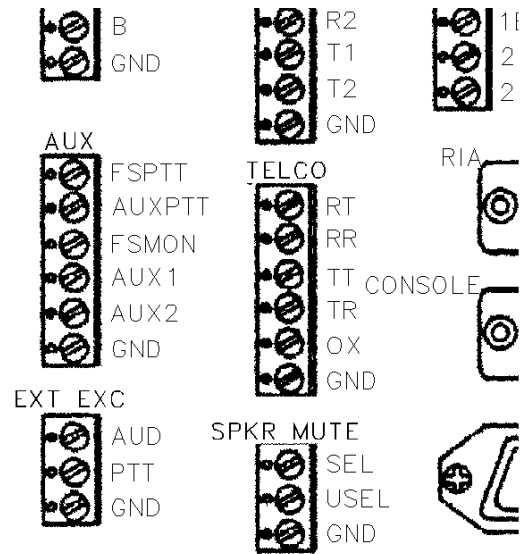
Figure 5-8 TELCO CONNECTION TO CIP PS
