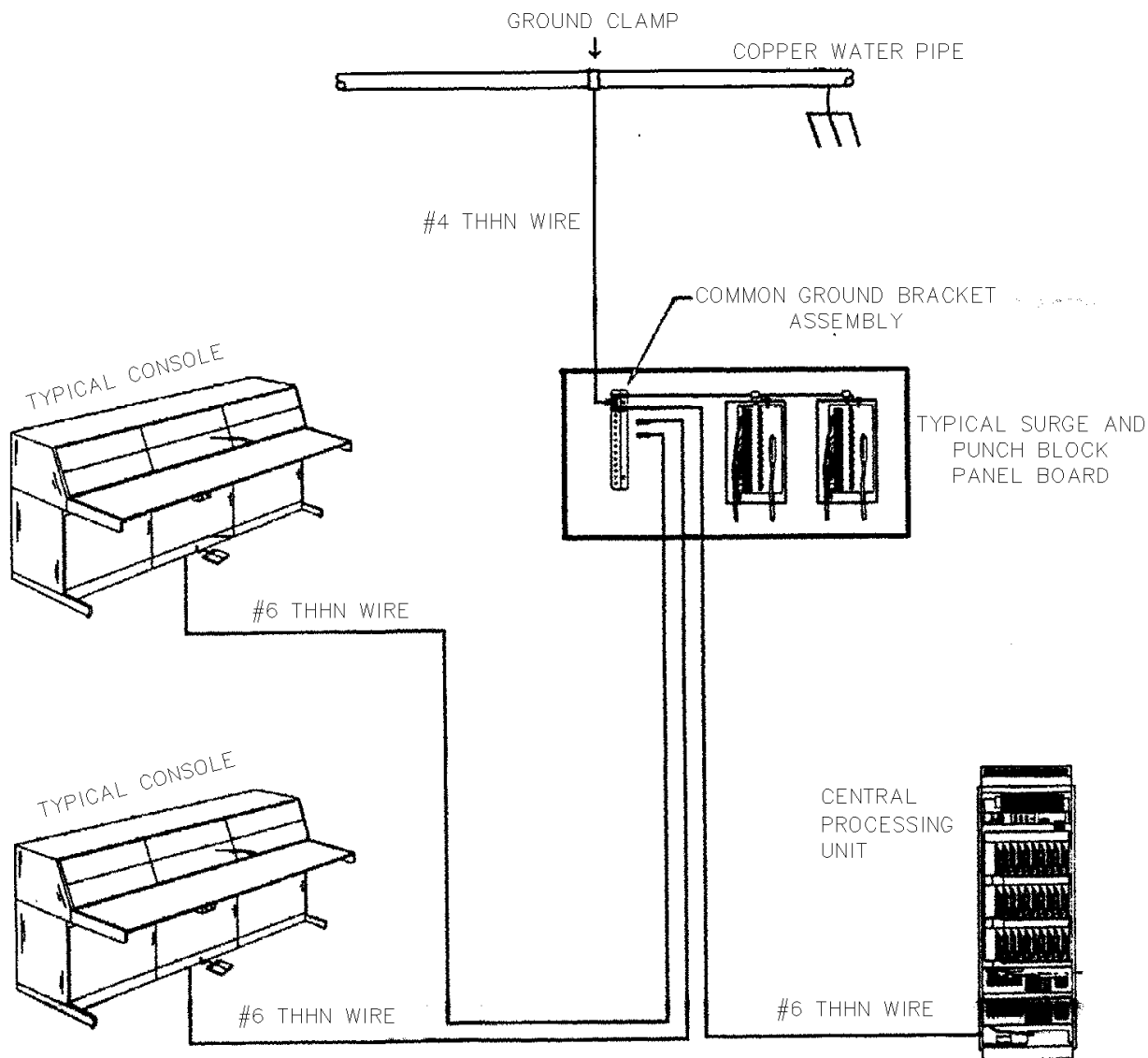
Figure 2-4 STAR GROUNDING CONFIGURATION
