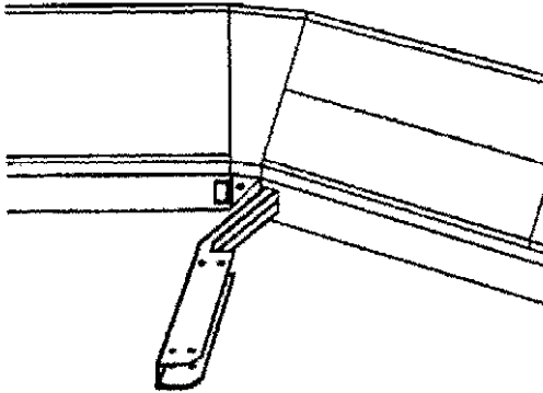
Figure 3-16 PIE SUPPORT RAIL MOUNTING
