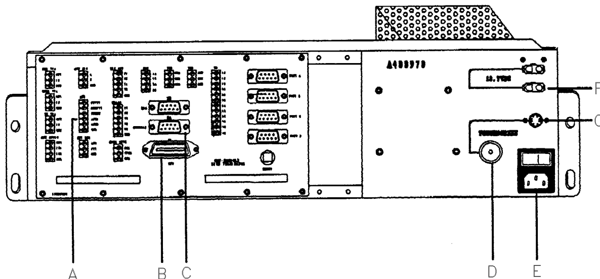
Figure 4-2 CIP POWER SUPPLY
