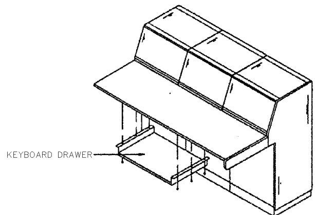
Figure 3-13 KEYBOARD DRAWER MOUNTING
