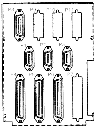
14 CARD SINGLE I/O PANEL
