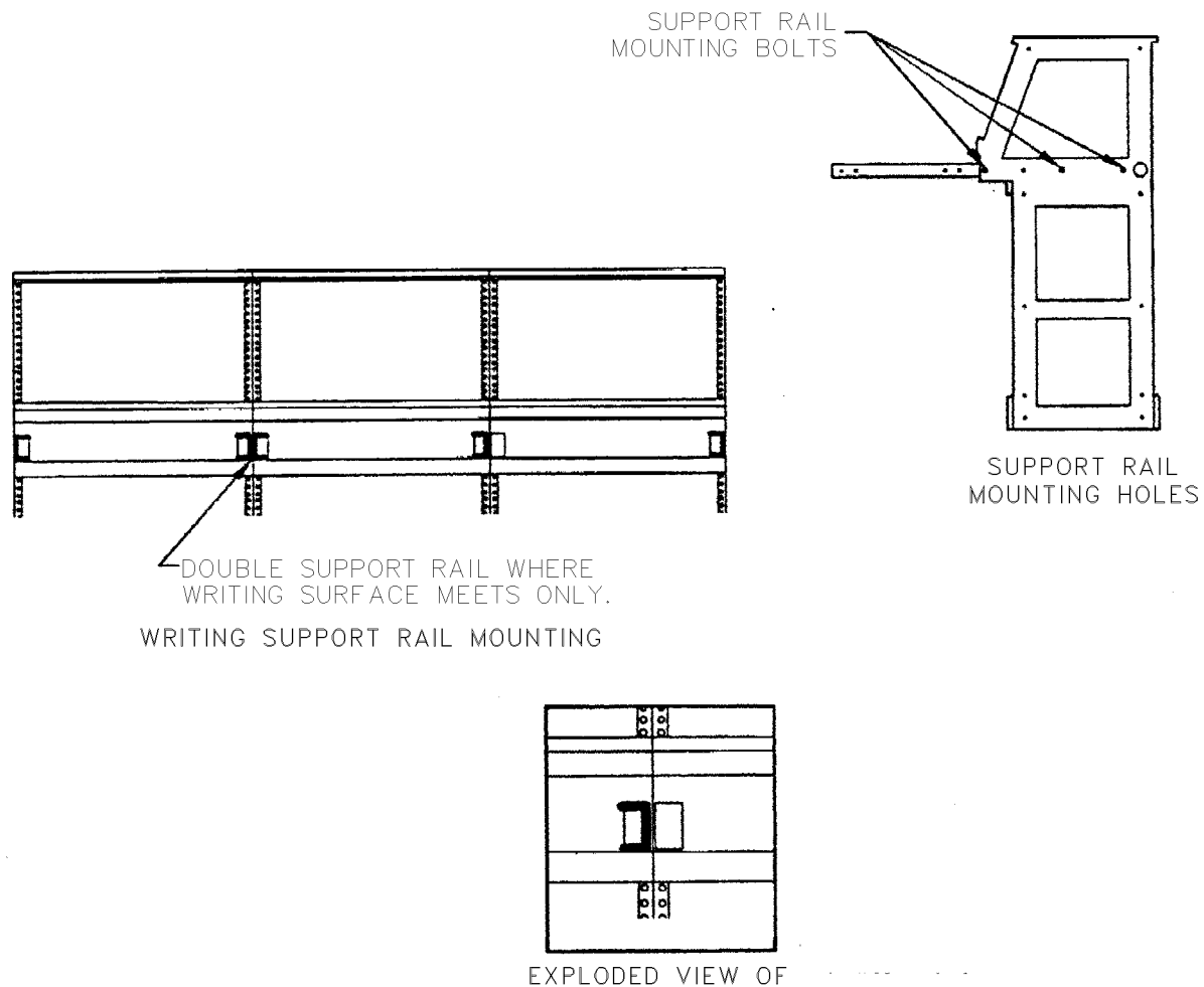
Figure 3-6 WRITING SUPPORT RAIL MOUNTING
