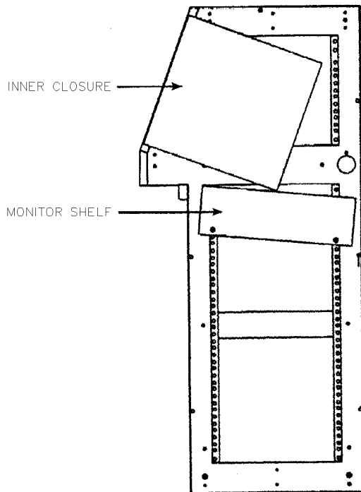
Figure 3-18 CRT MONITOR SHELF
