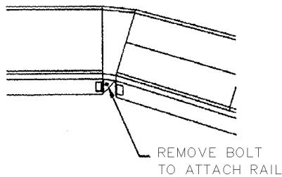
SUPPORT RAIL INSTALLATION ON 45° SECTION
