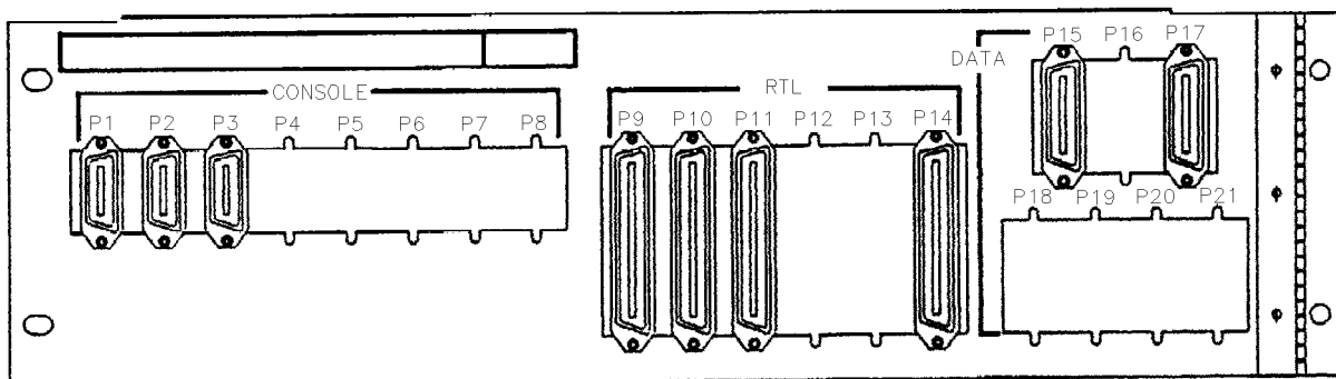
TO DISPATCH POSITIONS TO RADIO TIE LINES TO DATA TERMINALS 20 (or more) CARD CPP I/O PANEL
